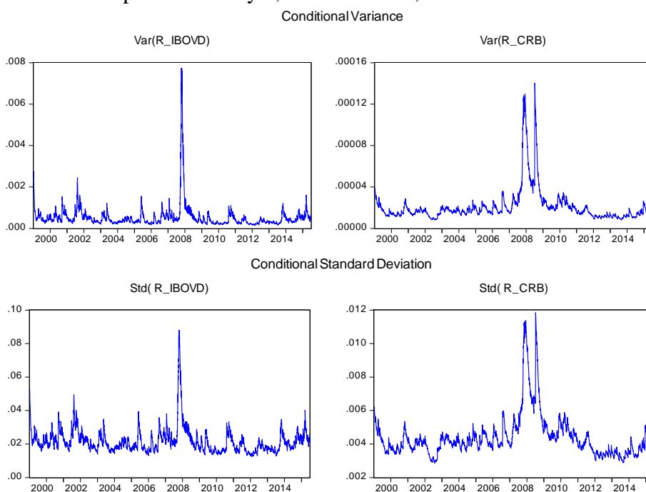
Figure 6. Conditional standard deviation and conditional variance of the Ibovespa returns in US$ and the CRB in the period January 3, 2000–June 30, 2016
