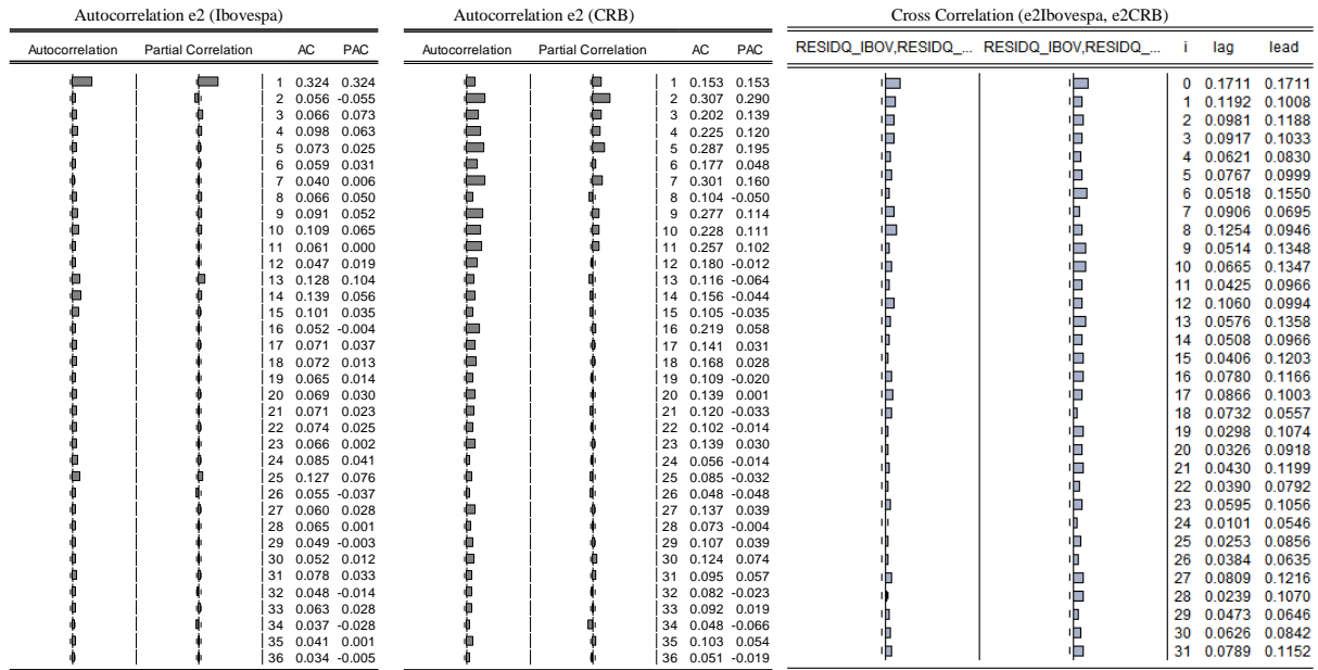
Figure 5. Squared-residual autocorrelations and squared-residual cross correlation between the Ibovespa in US$ and the CRB in the period January 3, 2000–June 30, 2016
