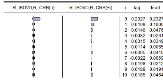
Figure 3. Cross-correlogram between CRB and Ibovespa in US$ in the period January 3, 2000–June 30, 2016
