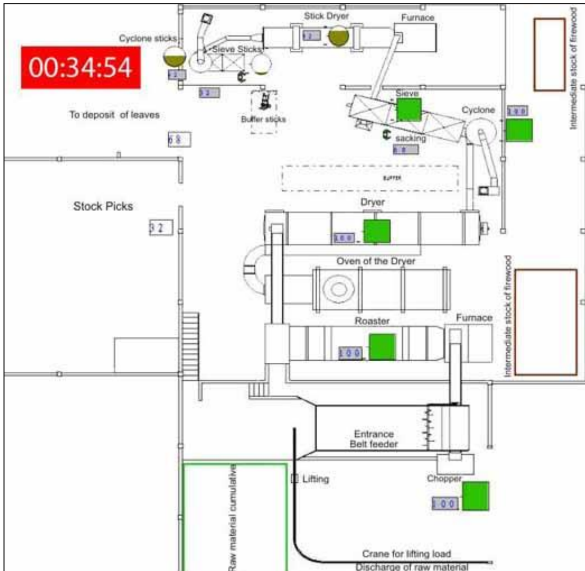
Figure 6 - Visualization of Simulation of Industrial Drying Yerba Mate of Instant T34
