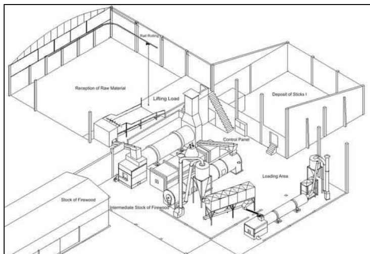
Figure 3 - Overview of the Unit for Industrial Drying Yerba Mate
